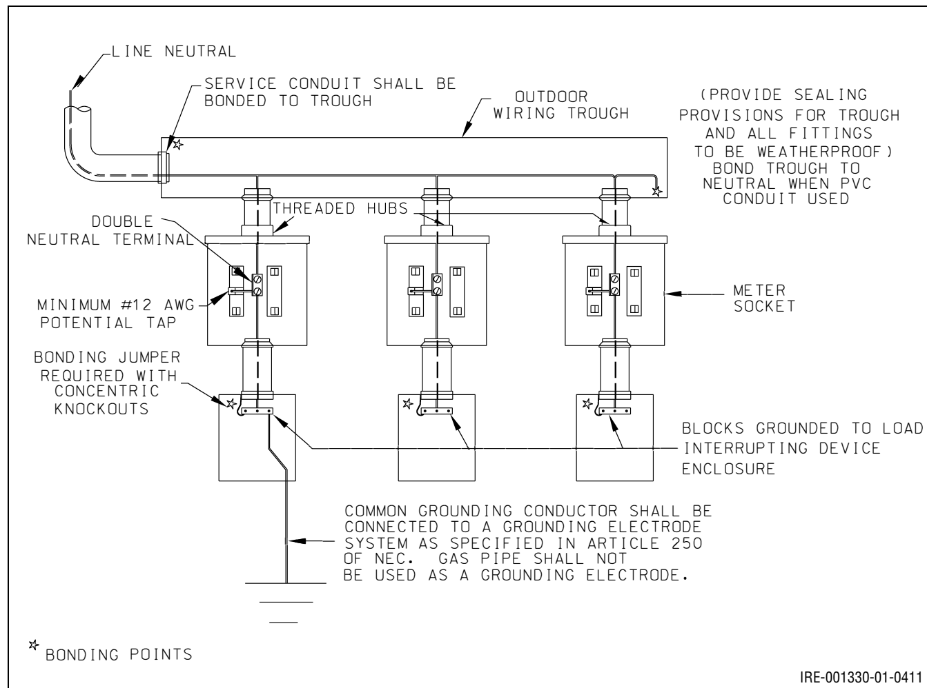
Figure 10.23: 120/208 or 120/240 V Service
