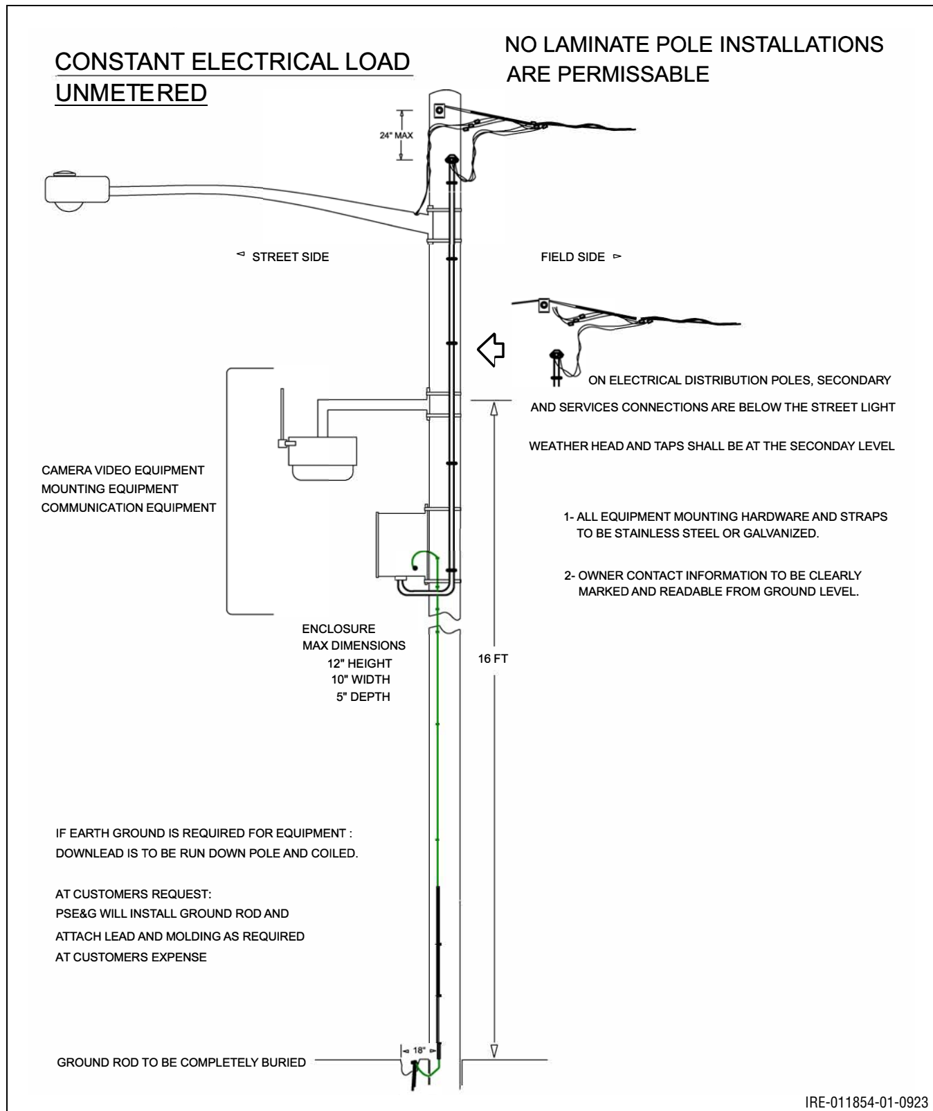
Figure 6.5: Video Equipment Installed on Wood or Composite Overhead Feed Street Lamp and Distribution Poles – Constant Electrical Load (Unmetered)
