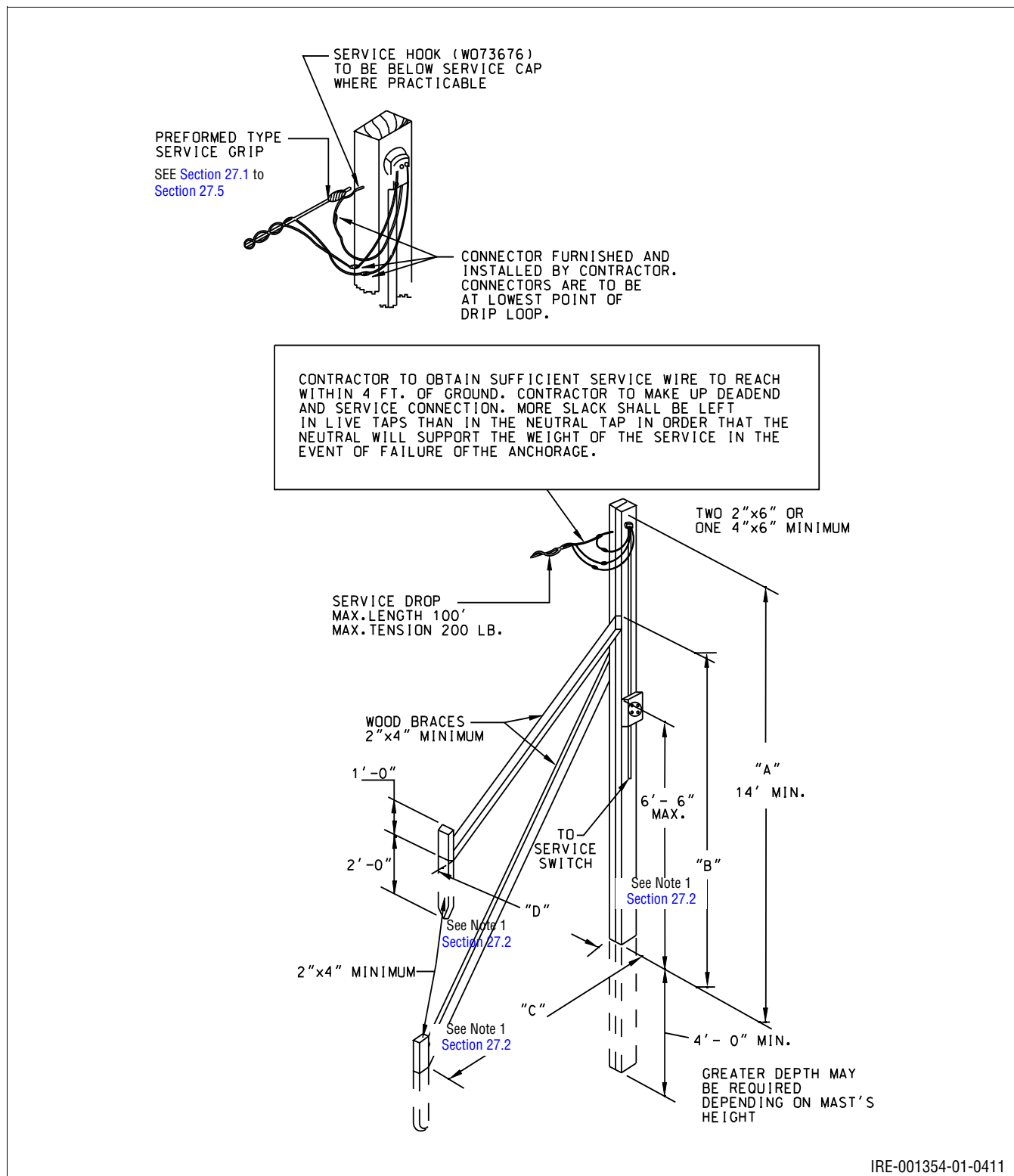
Figure 10.68: Minimum Requirements for a Temporary Service Mast
