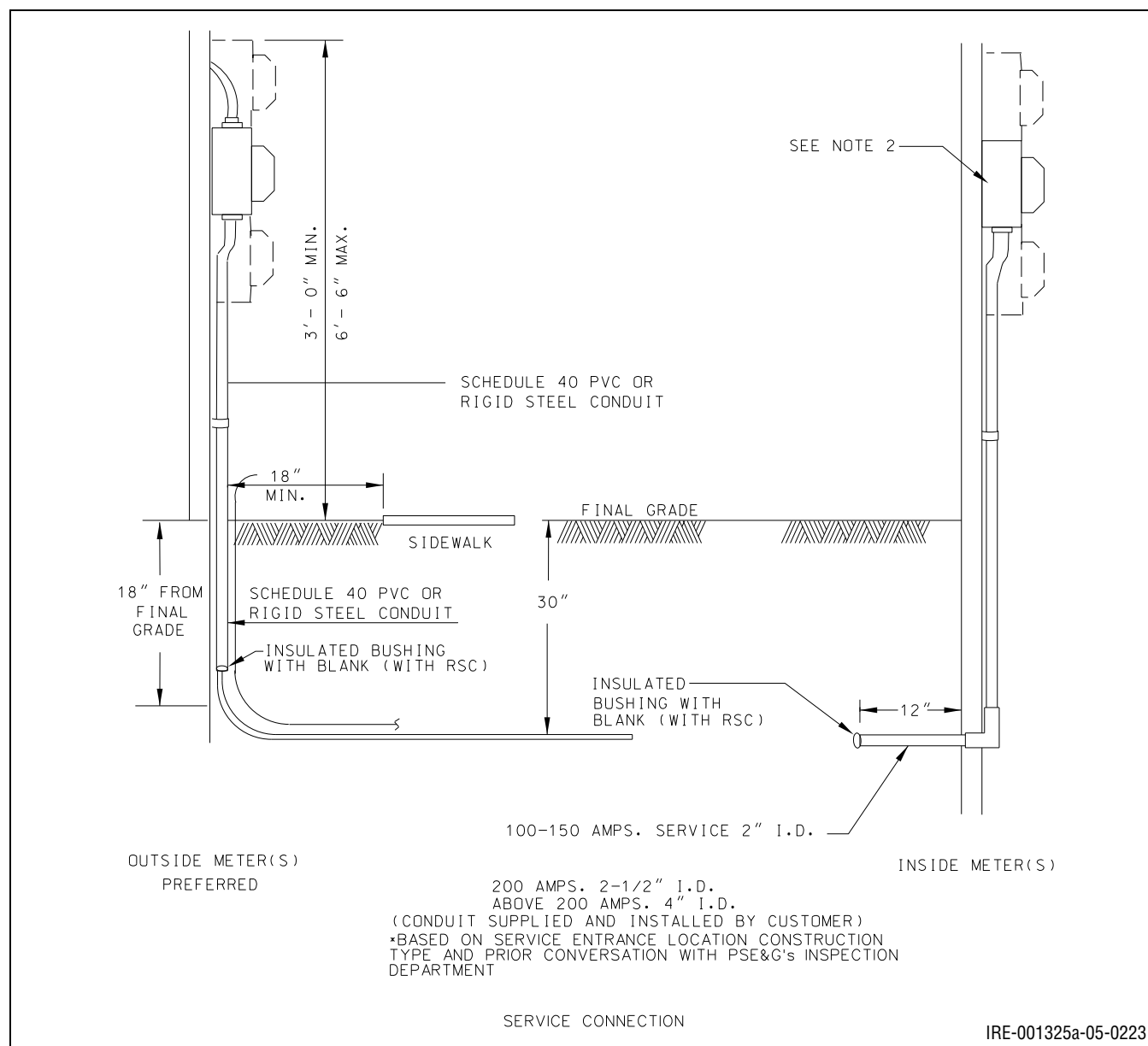
Figure 10.15: Service Connection
