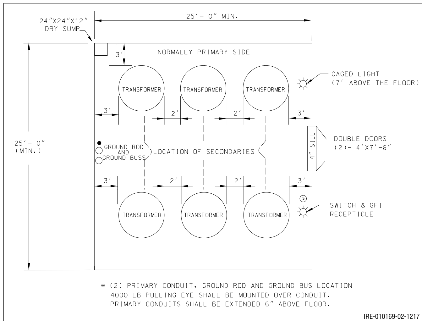
Figure 10.48: Transformer Vault Minimum Construction Dimensions Single – Up to Three 500 kVA Transformers Double – Up to Six 500 kVA Transformers
