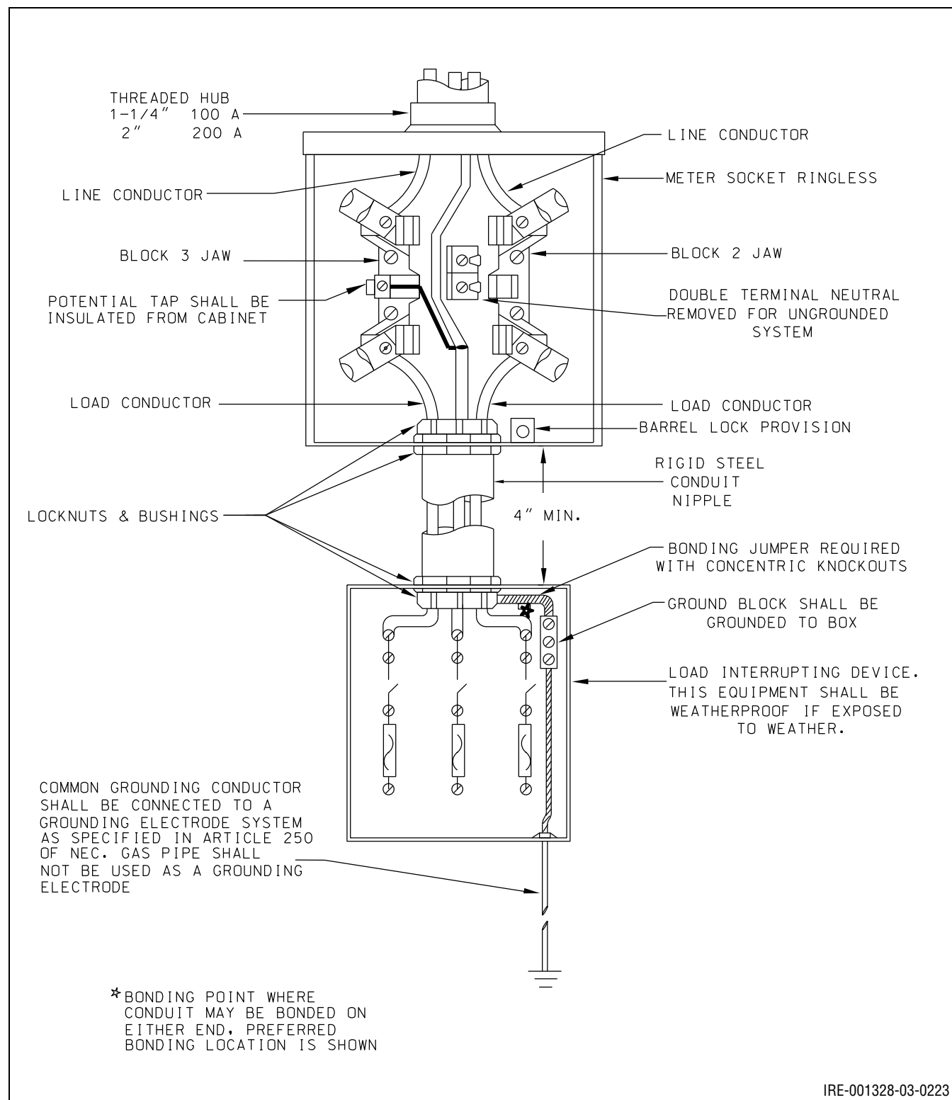
Figure 10.20: Three-Phase, Three-Wire, 240 V Service – Ungrounded System
