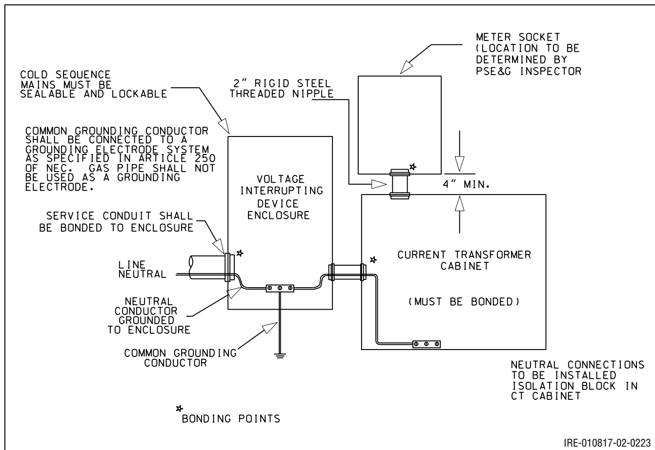
Figure 10.28: Grounding and Bonding CT Enclosure – Cold Sequence Bar Type CT
