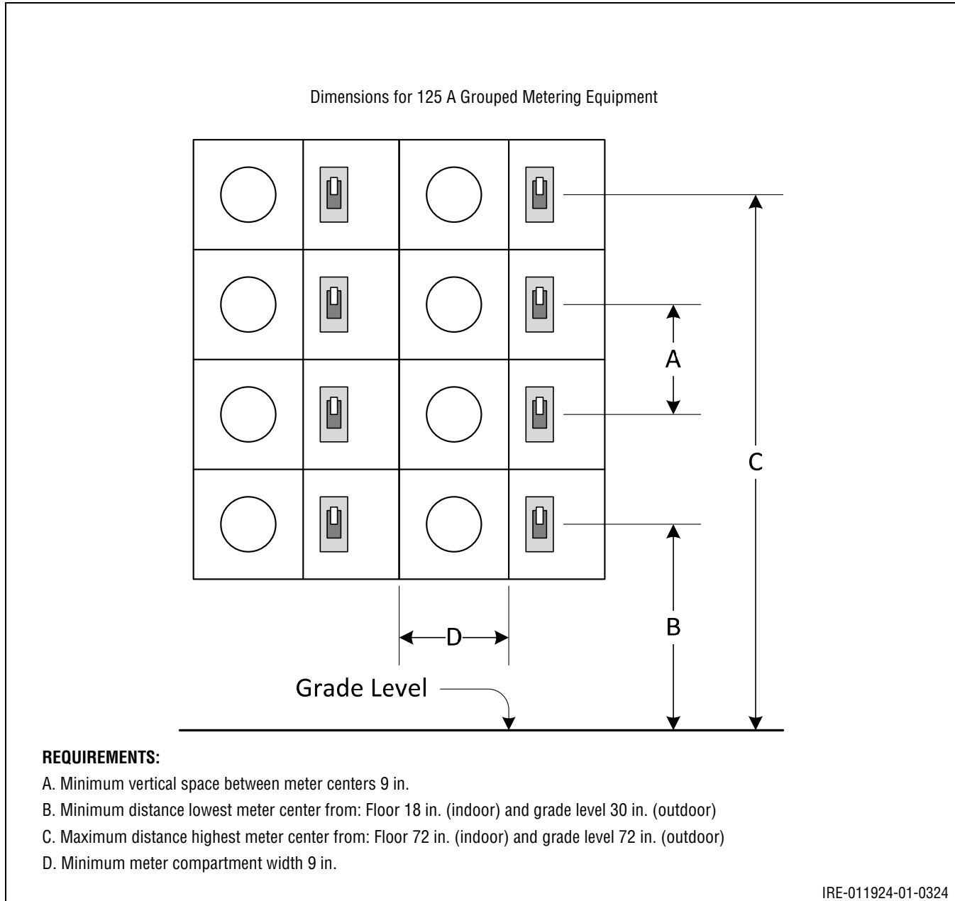
Figure 10.2: Exhibit 1 – Self-Contained, 125 A, Three-Wire 120/240 V, 120/208 V Network
