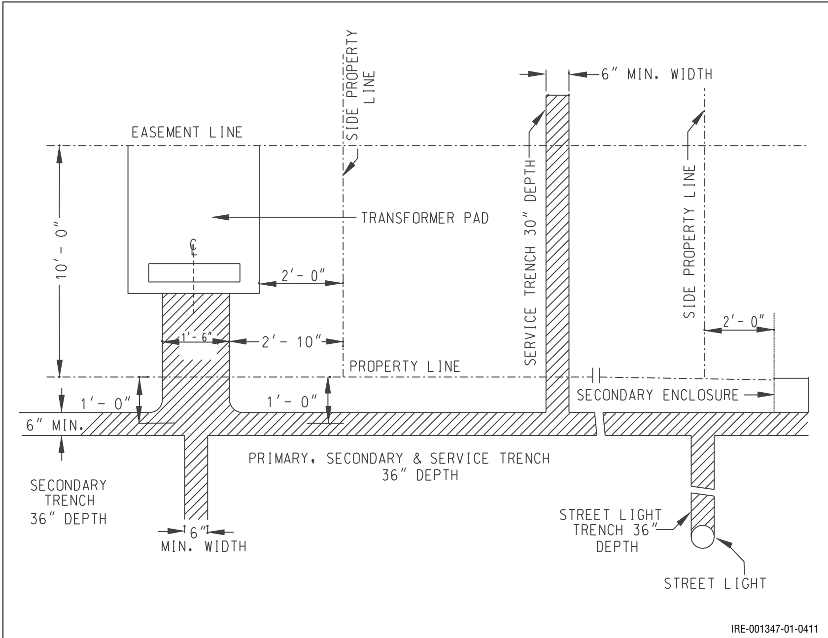
Figure 10.41: Single-Phase Padmounted Transformer Pads
