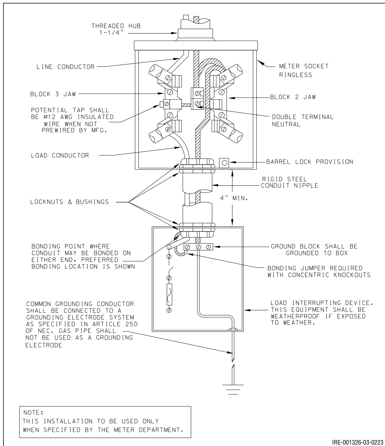
Figure 10.18: Single-Phase, Two-Wire 120 V for Two-Wire Socket Meter
