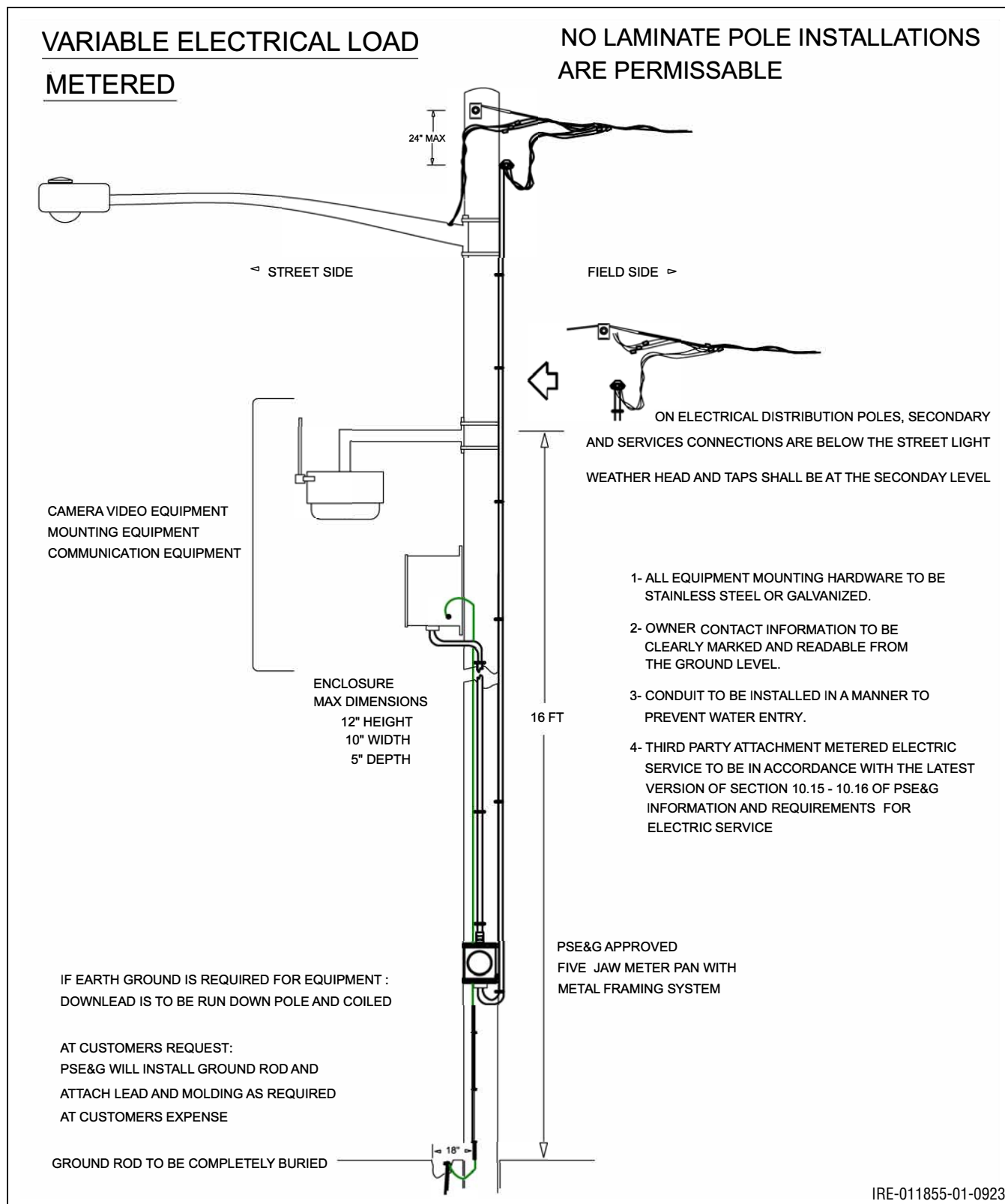
Figure 6.6: Video Equipment Installed on Wood or Composite Overhead Feed Street Lamp and Distribution Poles – Variable Electrical Load (Metered)
