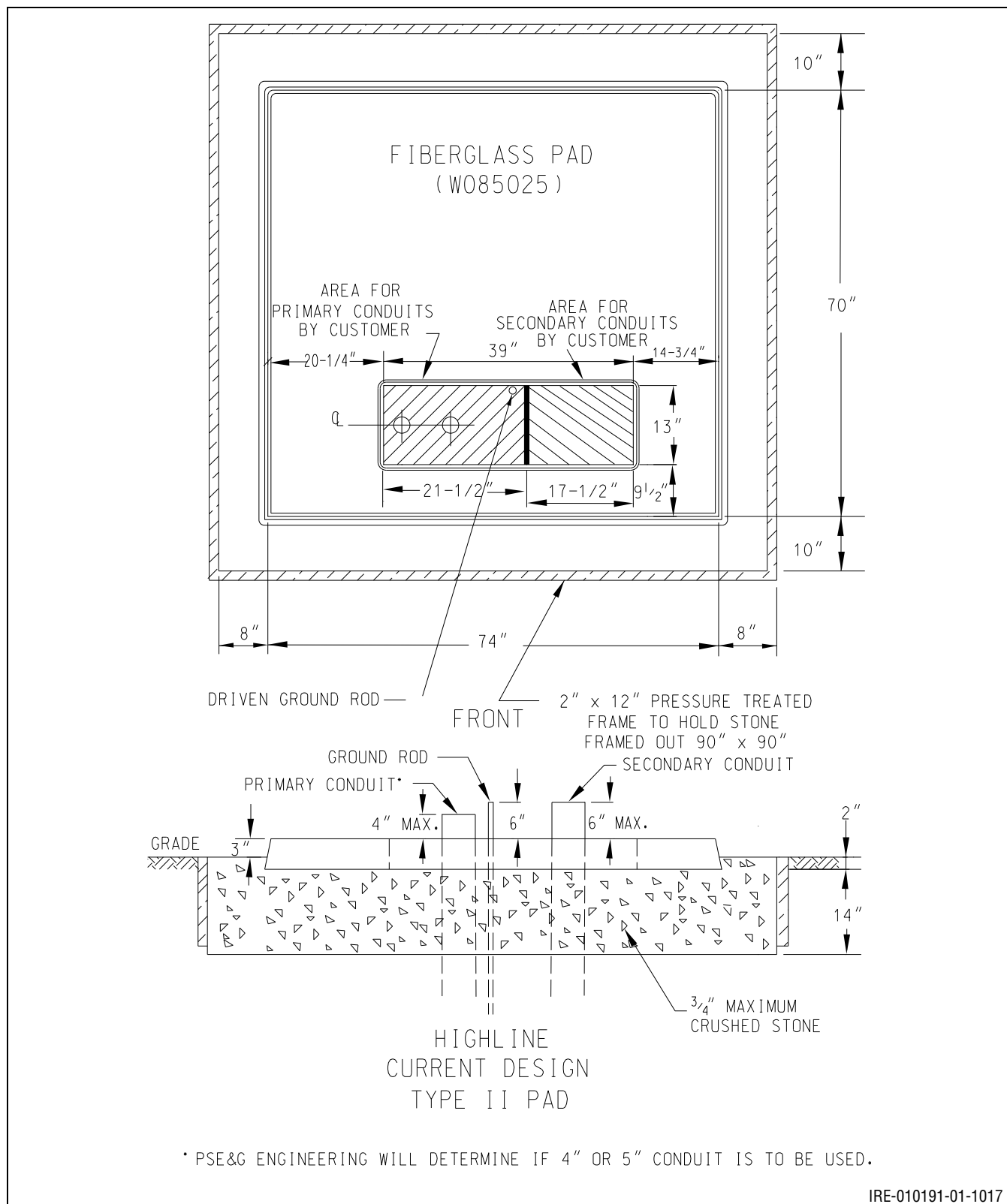
Figure 10.43: Fiberglass Pad Three-Phase Padmounted Transformers (300 kVA and below) – Type II (Highline Current Design Type II Pad)
