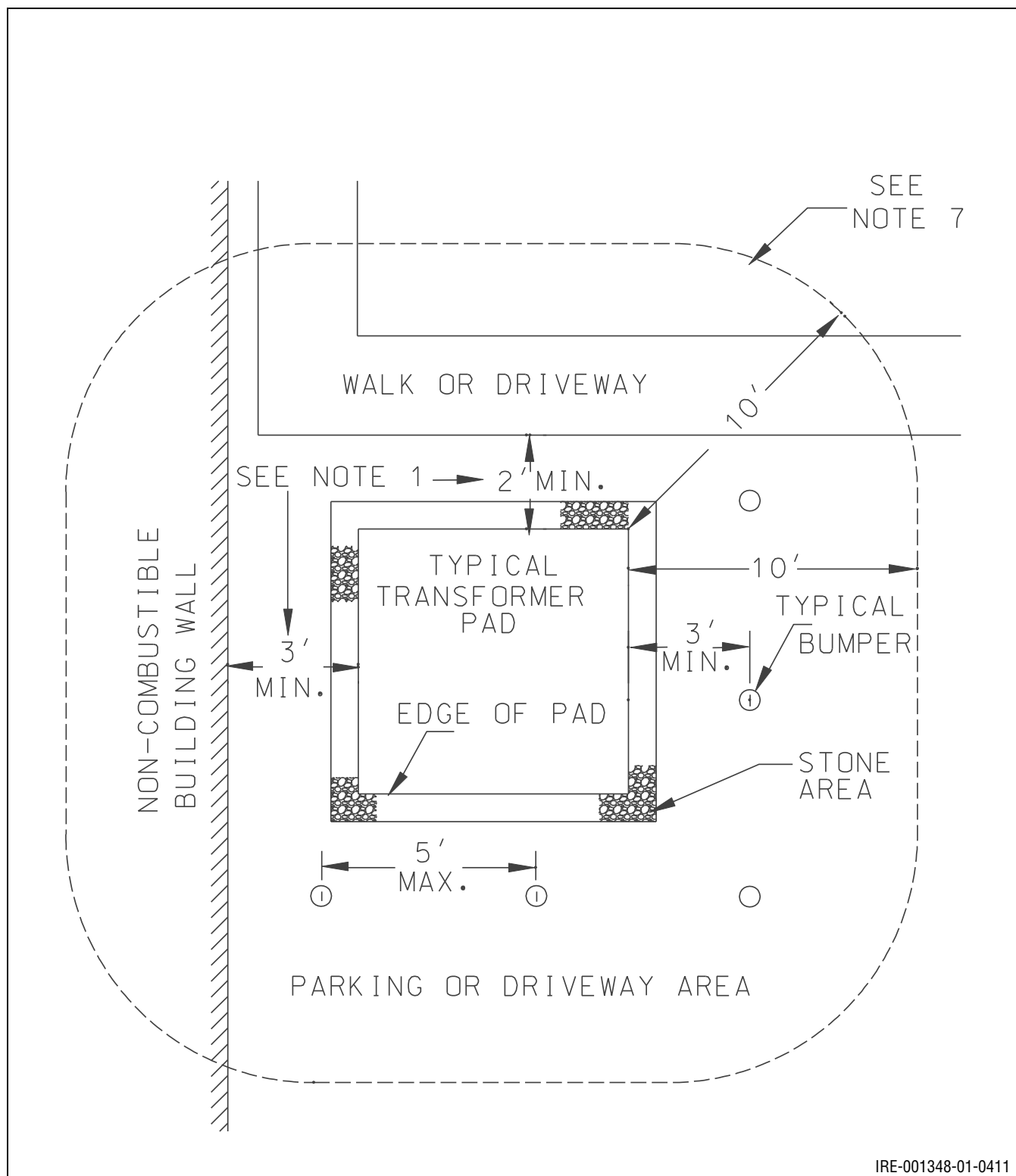
Figure 10.42: Three-Phase Padmounted Transformers
