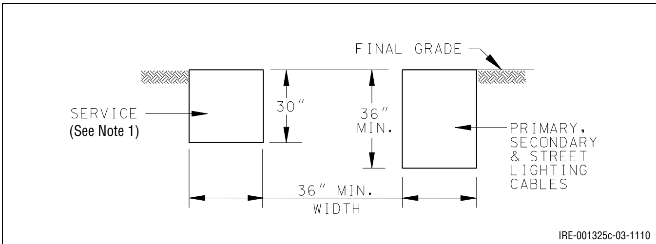
Figure 10.17: Standard Trenches
