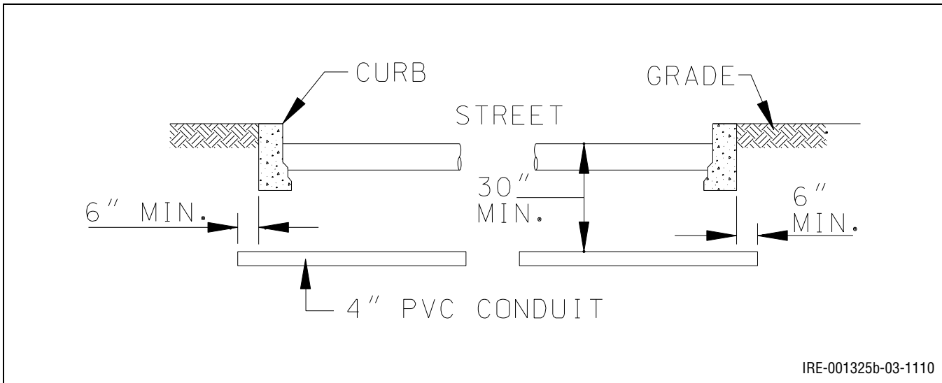
Figure 10.17: Standard Trenches
