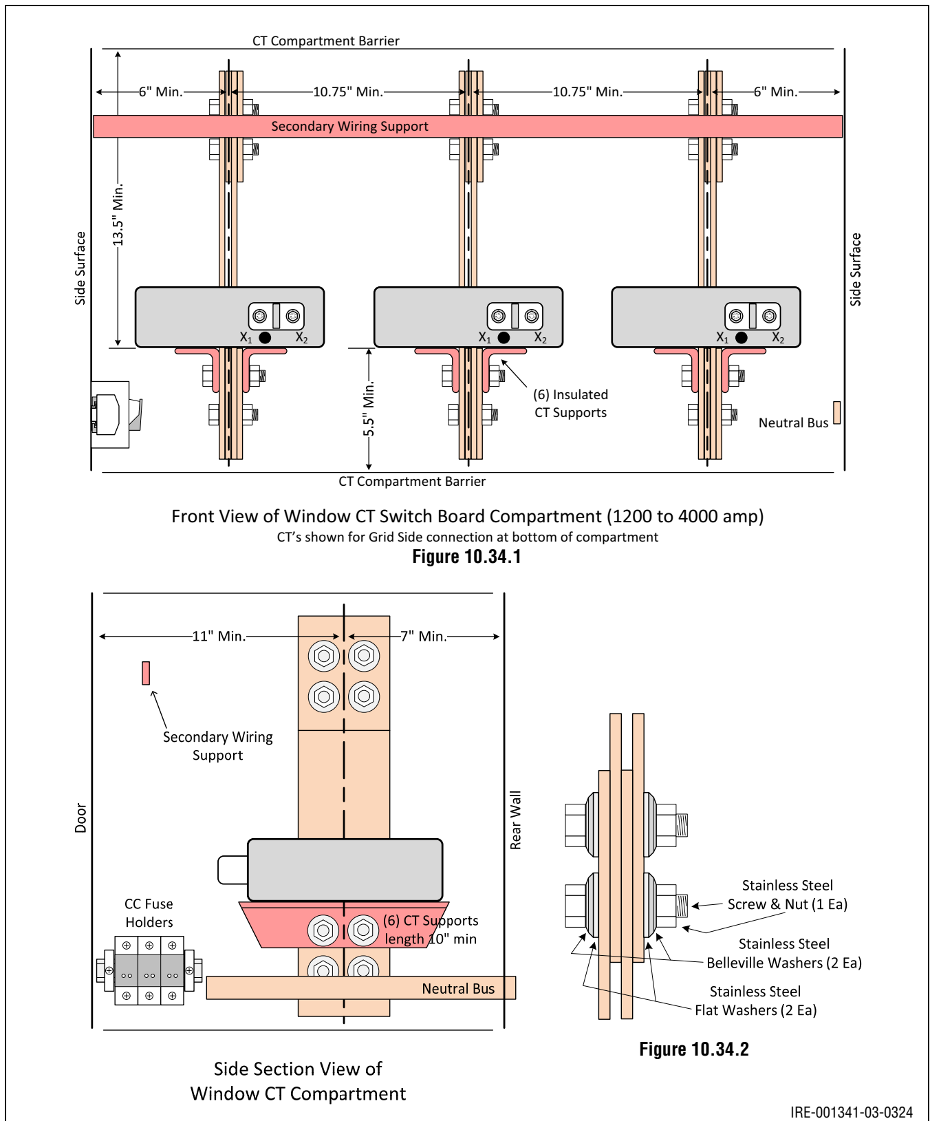
Figure 10.34: Window CT Compartment in Switchboard, 1200 to 4000 A, Voltage \leq 480
