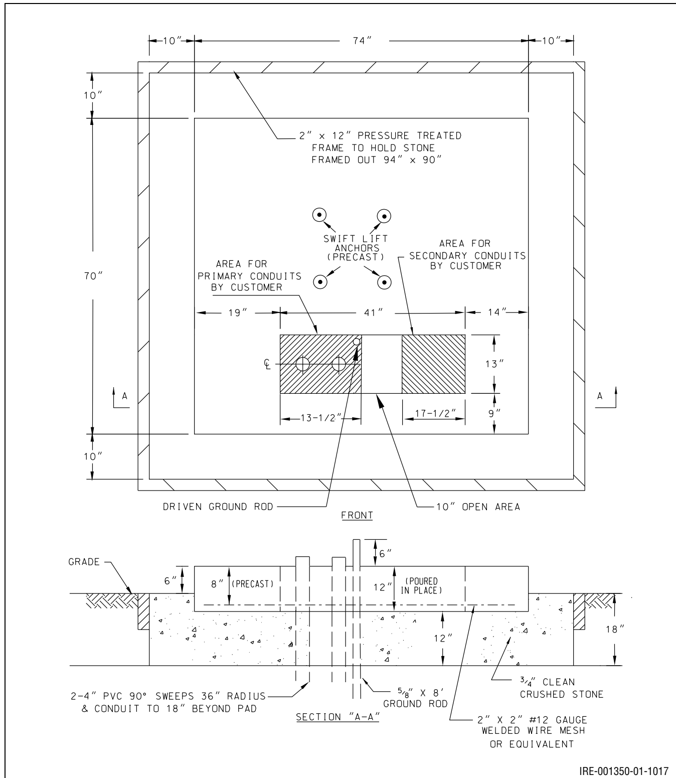
Figure 10.44: Three-Phase Padmounted Transformer – Type II-A (Concrete)
