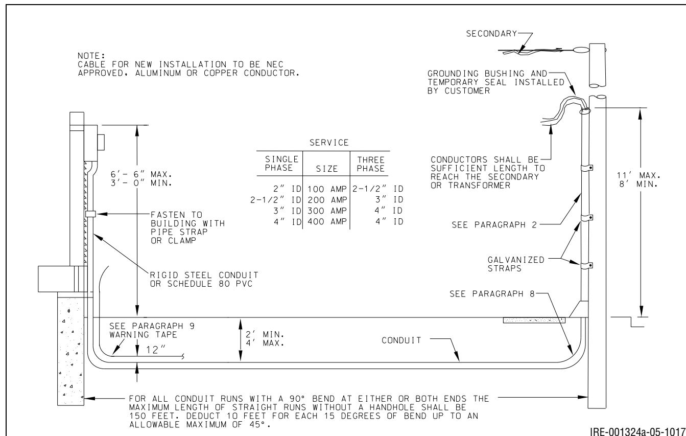
Figure 10.13: Service in Conduit
