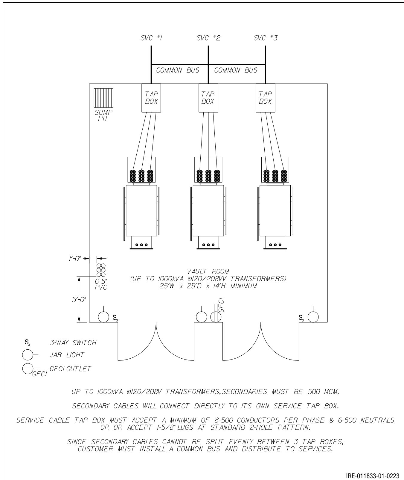
Figure 10.59: Up to 1,000 kVA at 120/208 V Transformer Vault Service to Three Tap Boxes Feeding Three Services – Customer Owned Common Bus
